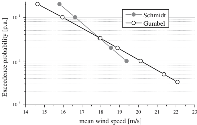
Figure 1. Extrapolated mean wind speeds for selected return periods up to 100 years (following Schmidt) and 300 years (following Gumbel).
